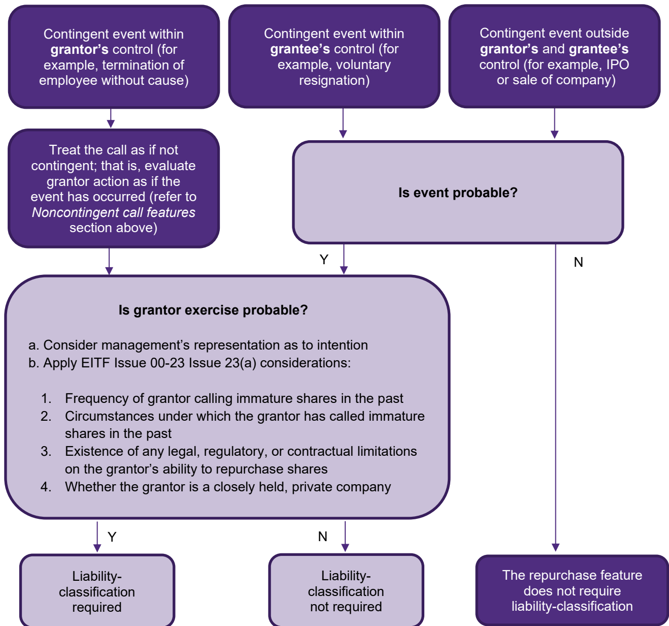
Figure 3.5: Evaluating contingent call features on immature shares at fair value
