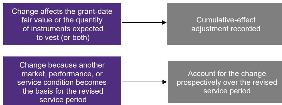
Figure 6.2 – Change in initial estimate of the requisite service period
